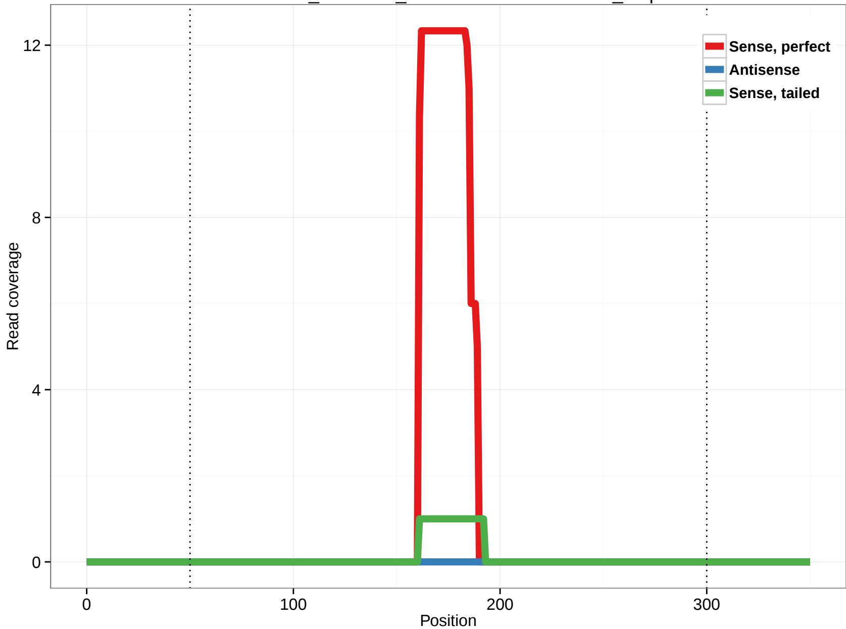
ornAna1_ensGene_ENSOANT00000015241_0.3p
