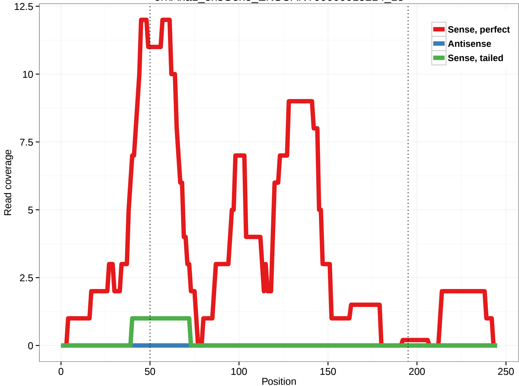
ornAna1_ensGene_ENSOANT00000015214_18
