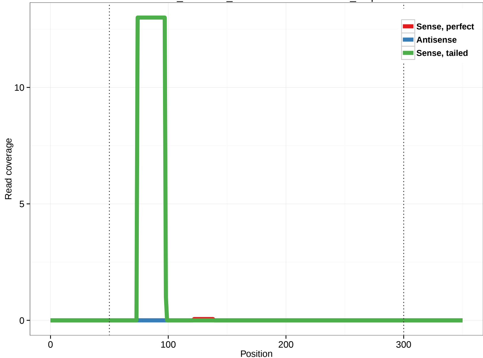
ornAna1_ensGene_ENSOANT00000015208_0.5p
