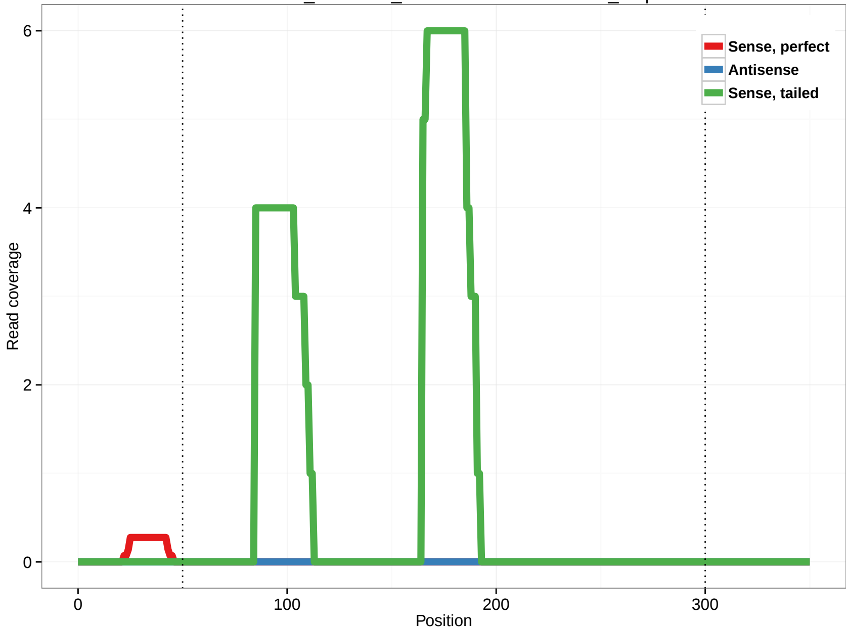
ornAna1_ensGene_ENSOANT00000015205_8.3p
