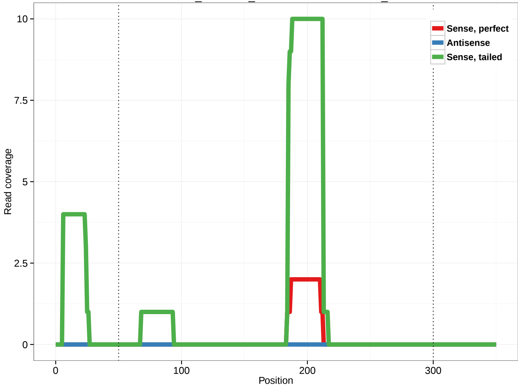
ornAna1_ensGene_ENSOANT00000015126_10
