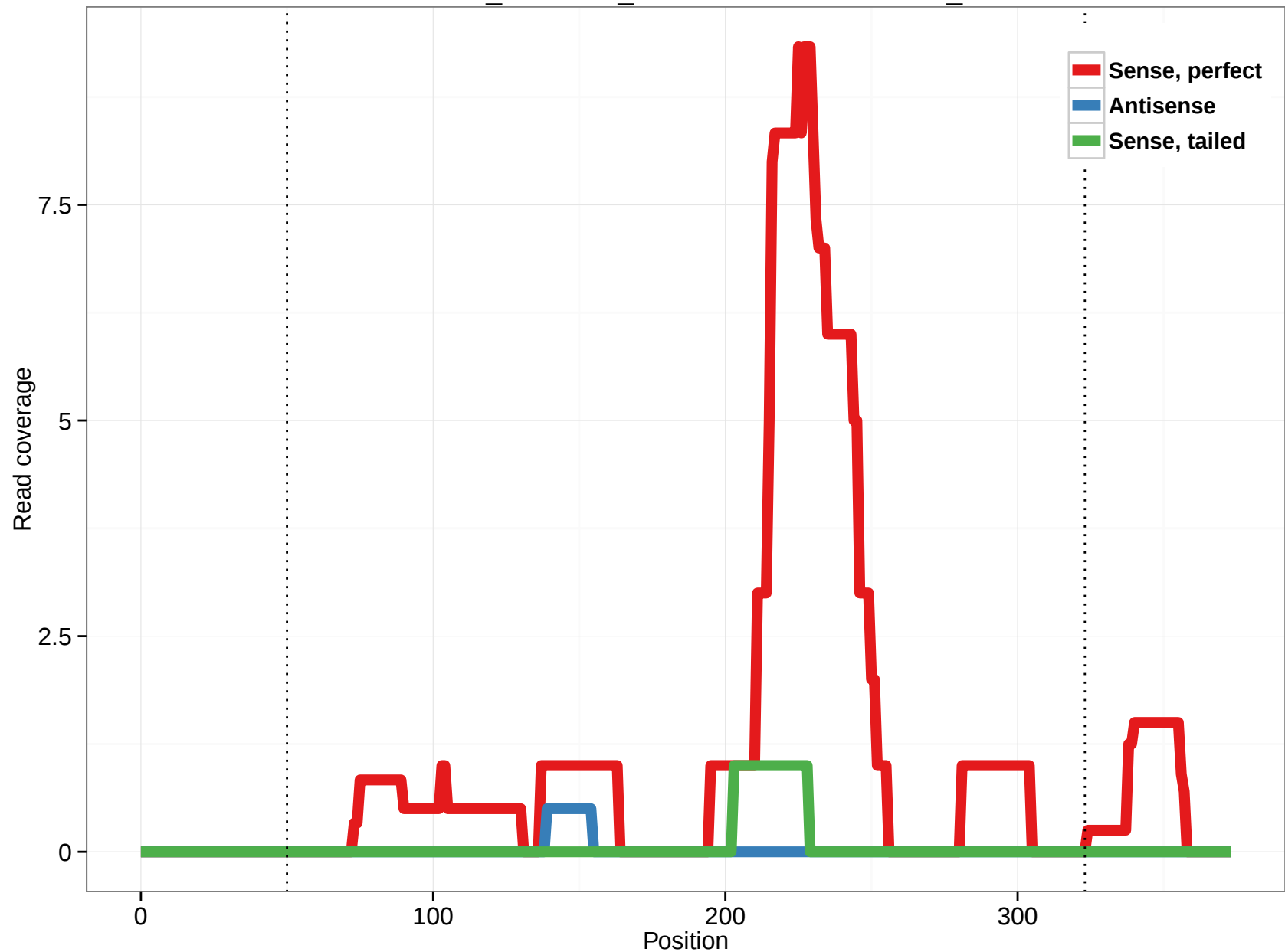
ornAna1_ensGene_ENSOANT00000015079_12
