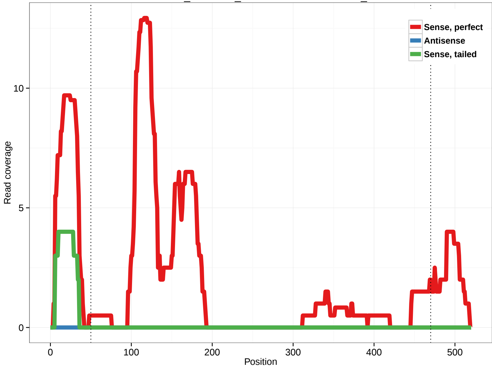
ornAna1_ensGene_ENSOANT00000015079_10
