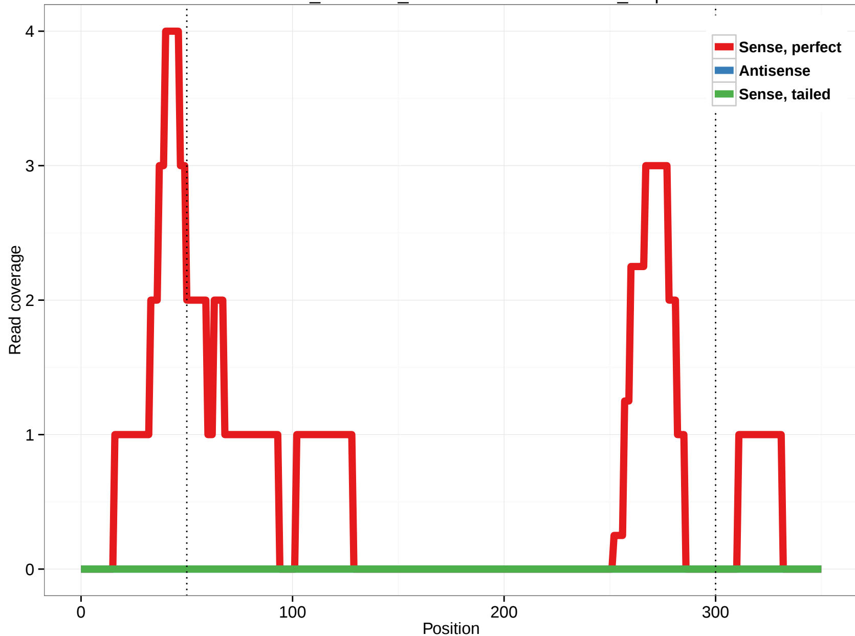
ornAna1_ensGene_ENSOANT00000015012_3.5p
