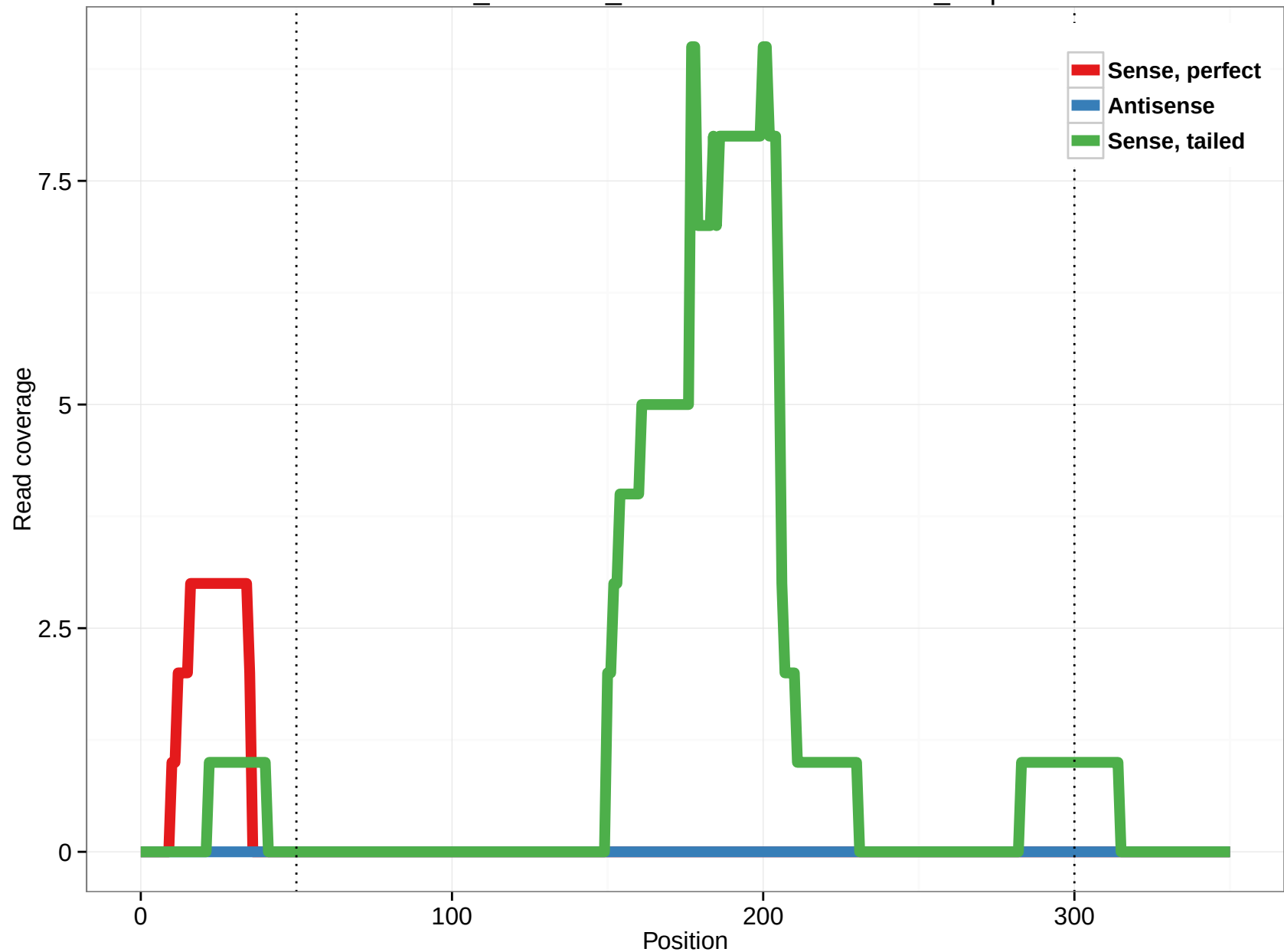
ornAna1_ensGene_ENSOANT00000015010_0.5p
