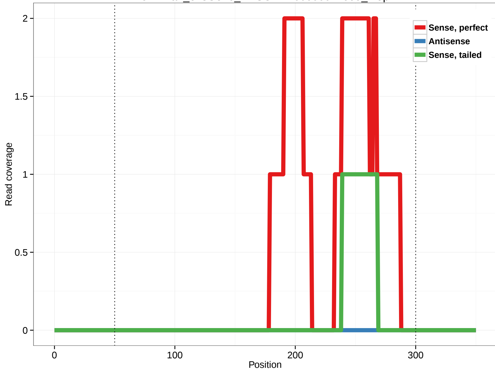
ornAna1_ensGene_ENSOANT00000014999_4.5p
