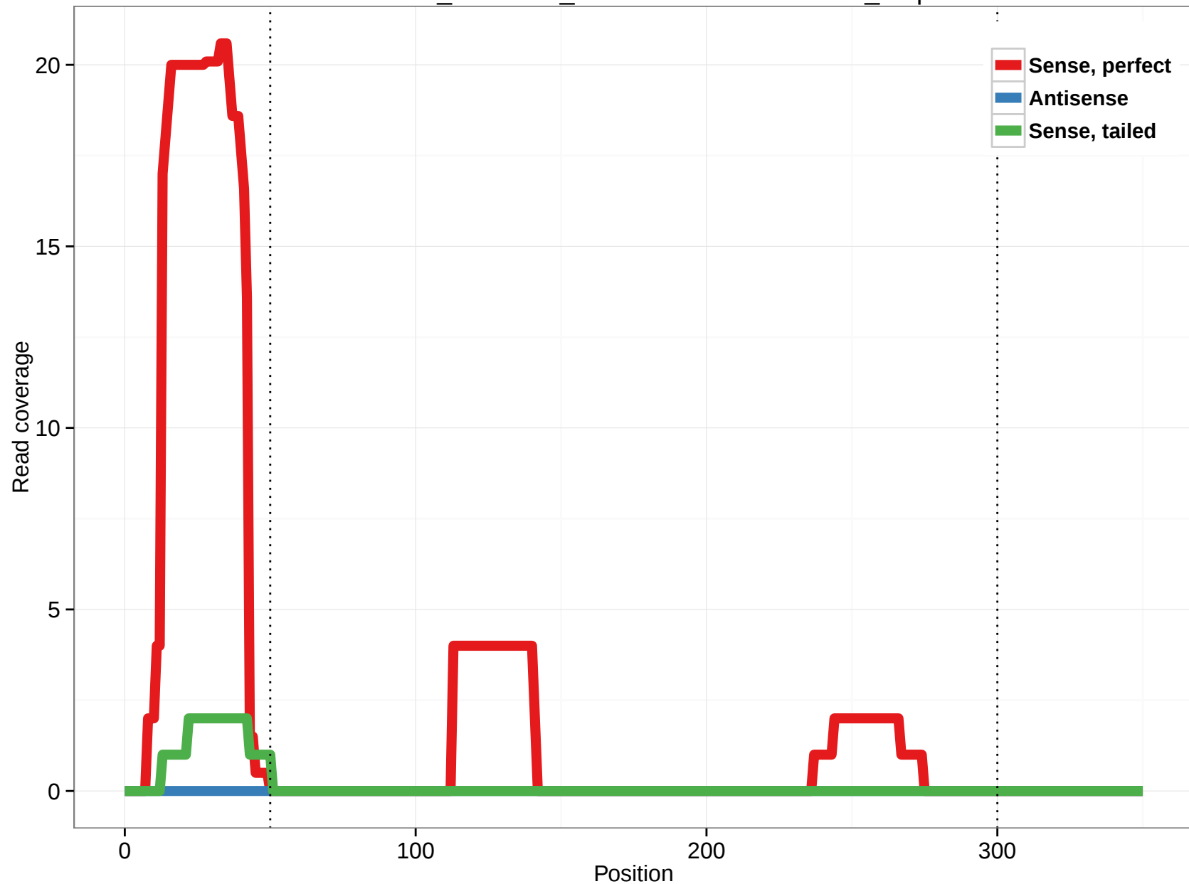
ornAna1_ensGene_ENSOANT00000014999_2.5p
