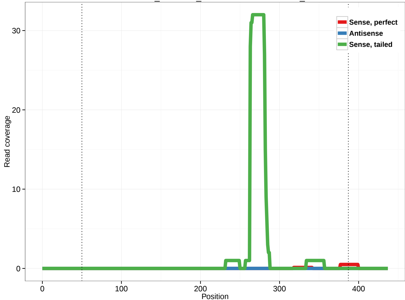
ornAna1_ensGene_ENSOANT00000014988_4
