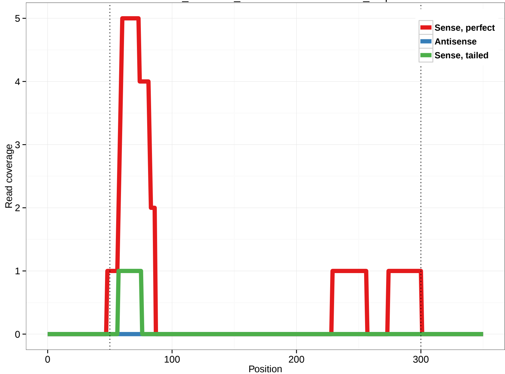
ornAna1_ensGene_ENSOANT00000014967_3.3p
