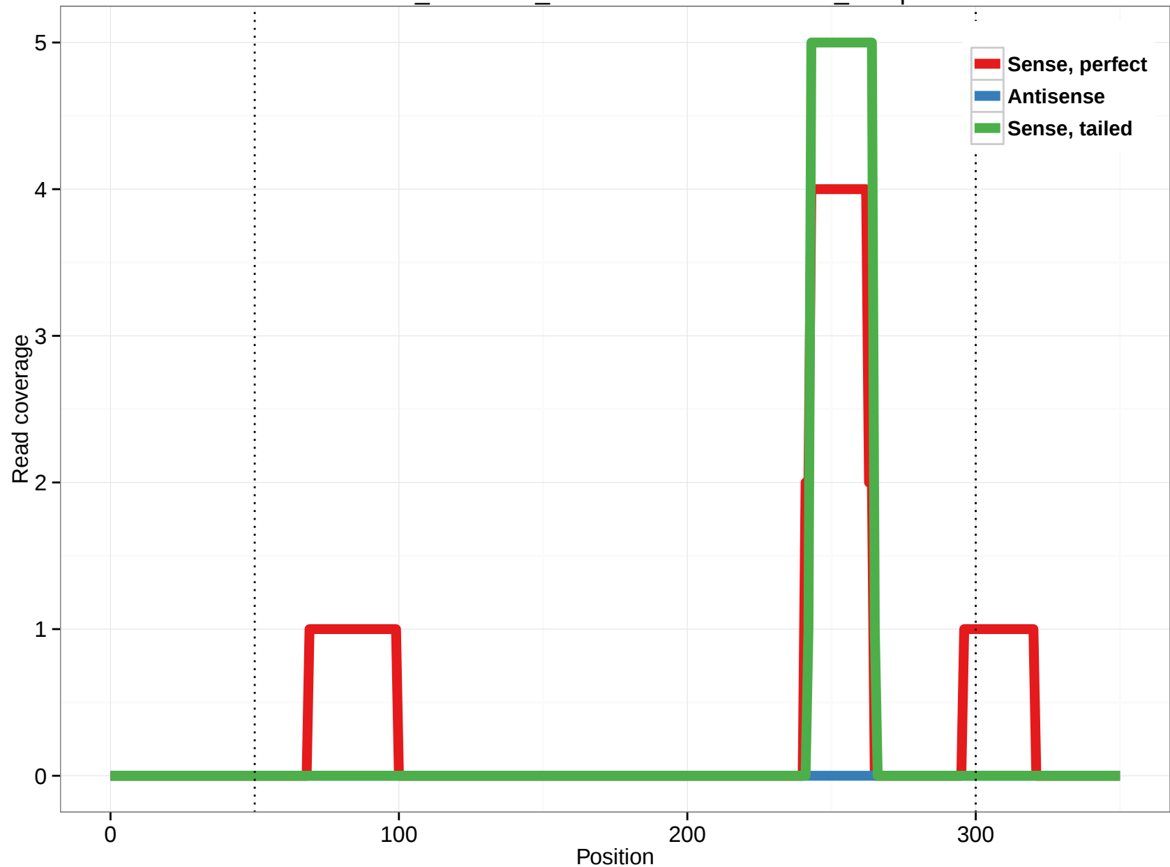
ornAna1_ensGene_ENSOANT00000014953_14.3p
