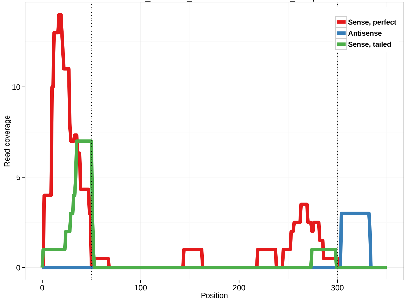
ornAna1_ensGene_ENSOANT00000014946_18.5p
