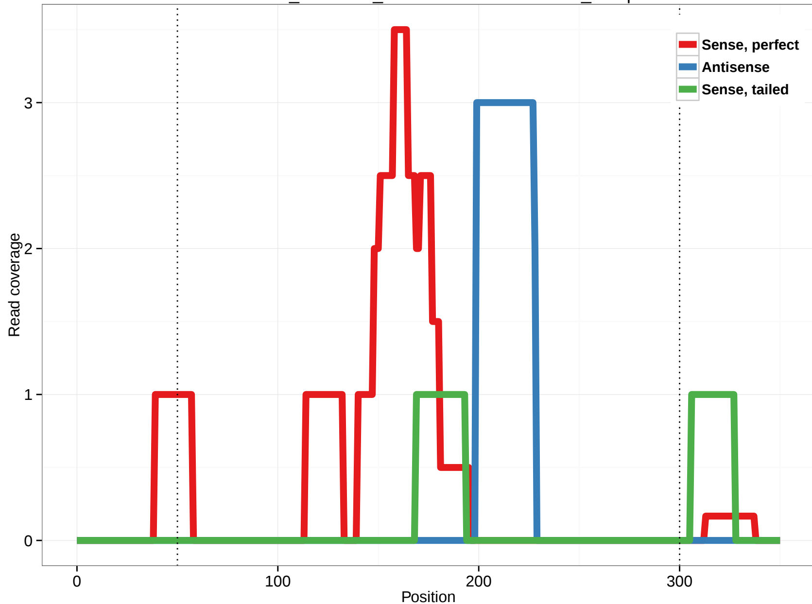
ornAna1_ensGene_ENSOANT00000014945_18.5p
