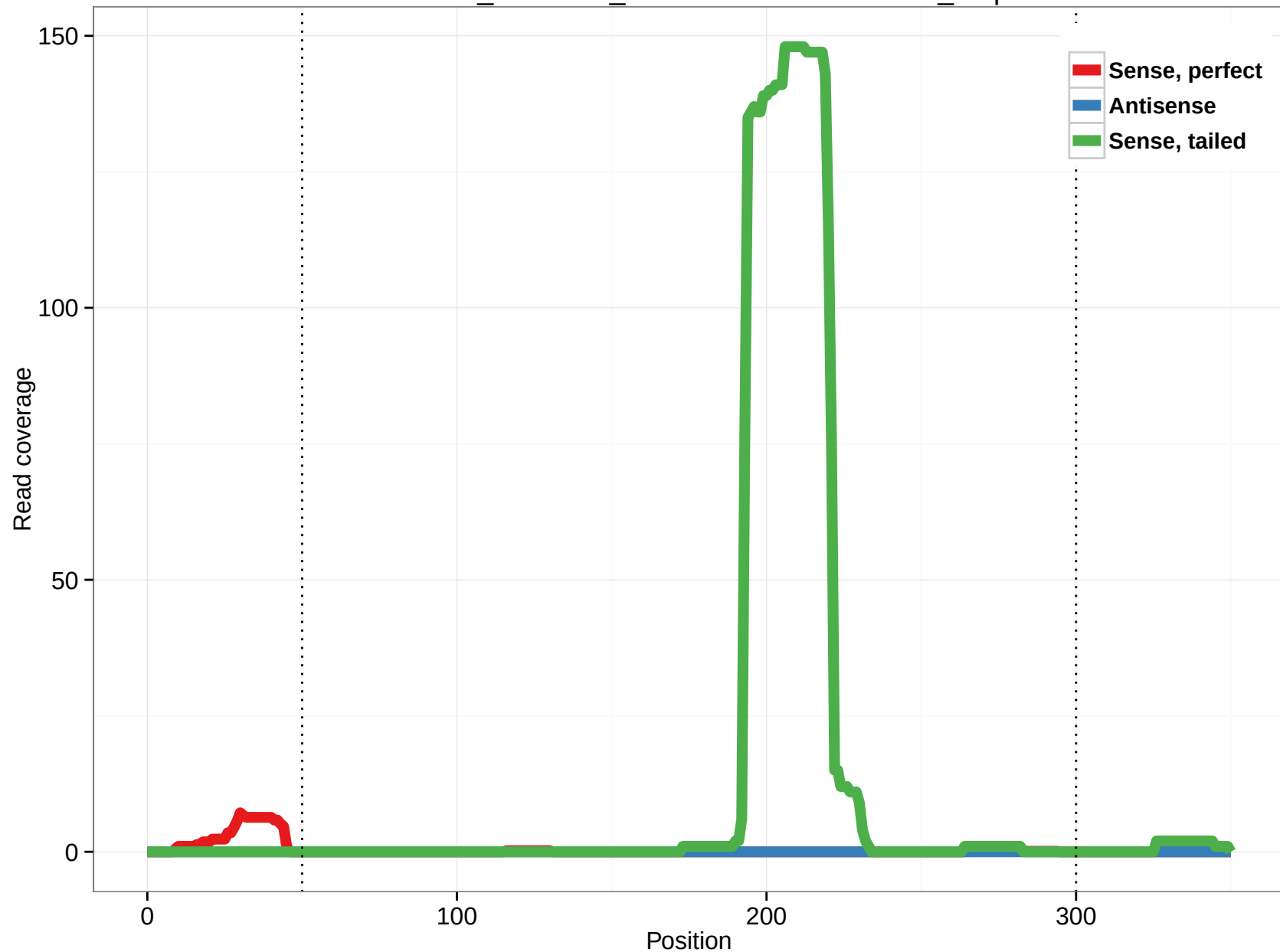
ornAna1_ensGene_ENSOANT00000014875_0.5p
