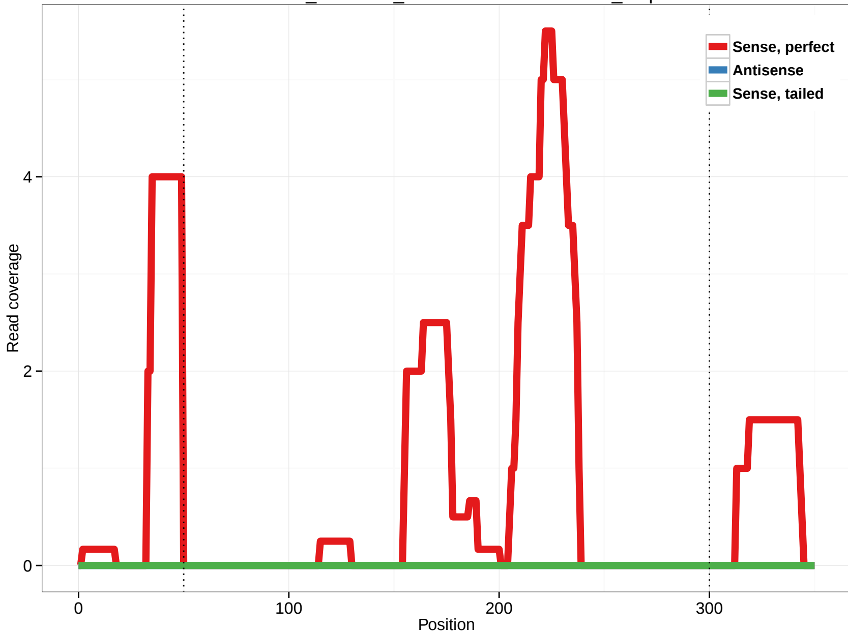
ornAna1_ensGene_ENSOANT00000014798_1.5p
