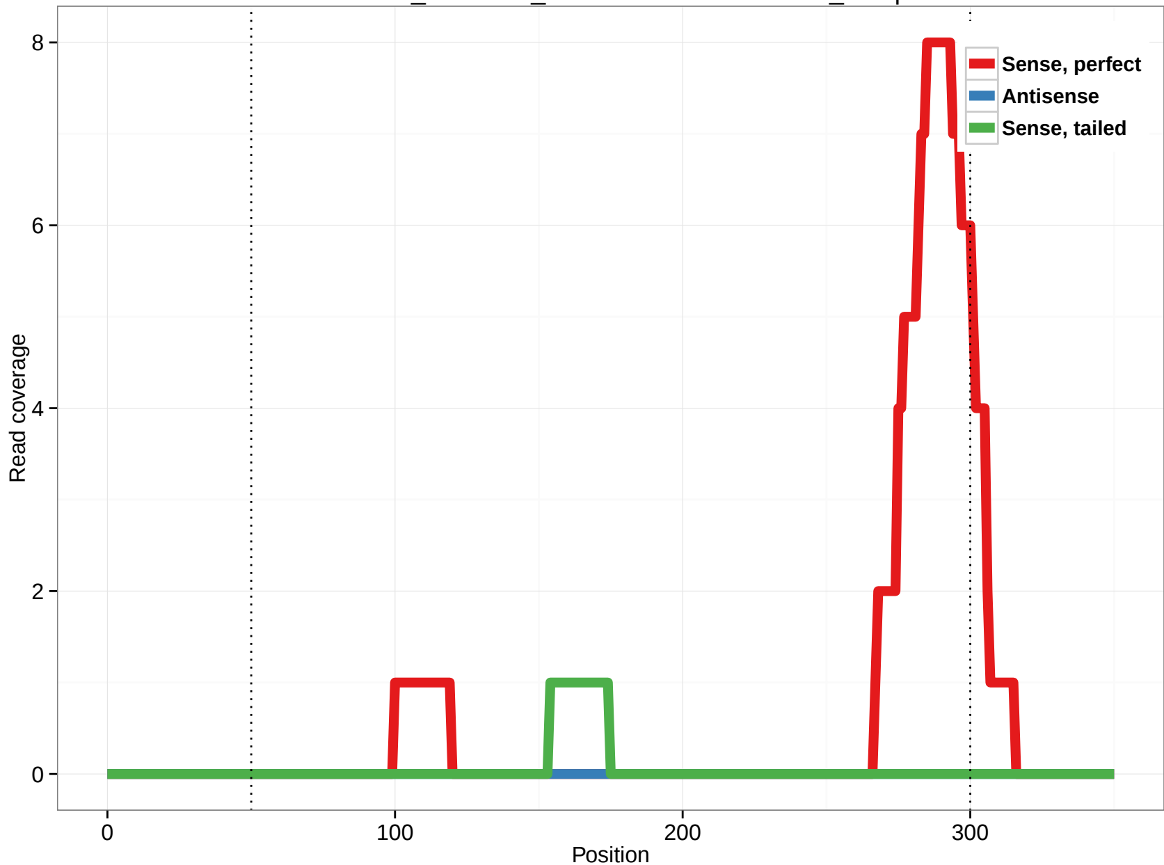
ornAna1_ensGene_ENSOANT00000014796_40.5p
