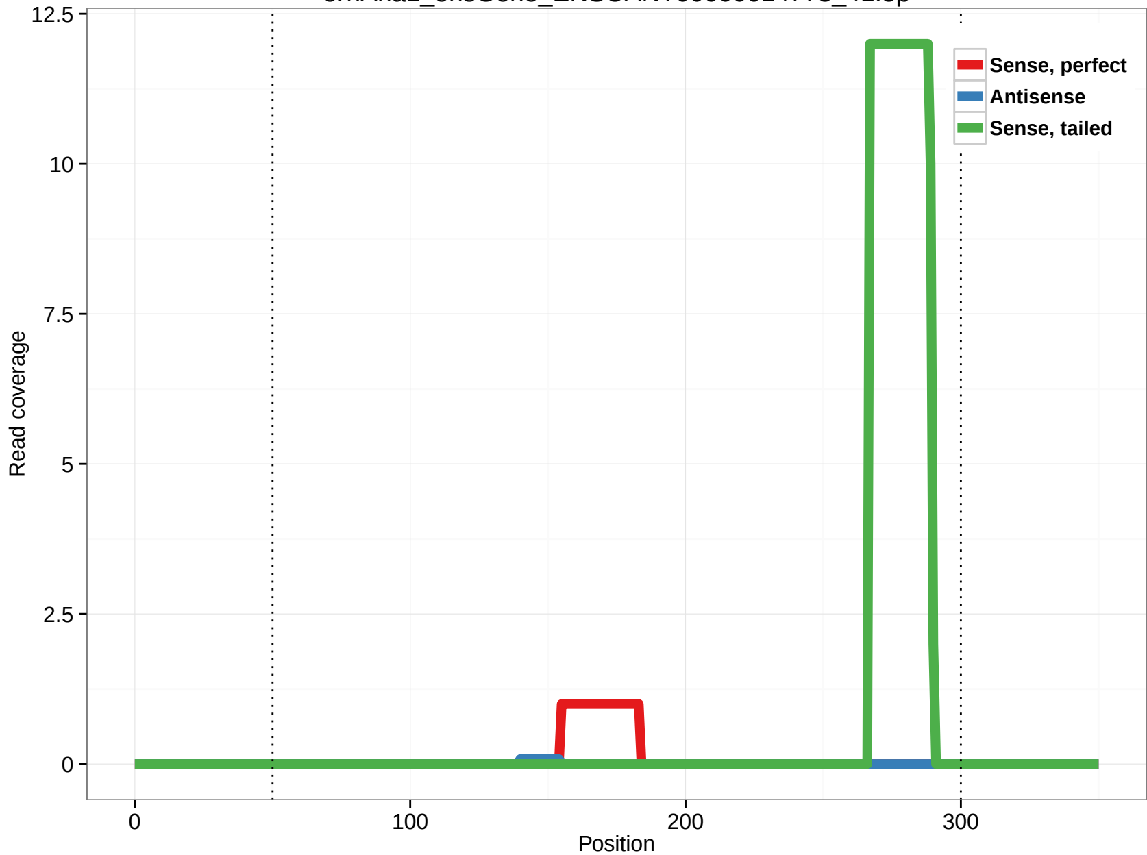
ornAna1_ensGene_ENSOANT00000014773_41.5p
