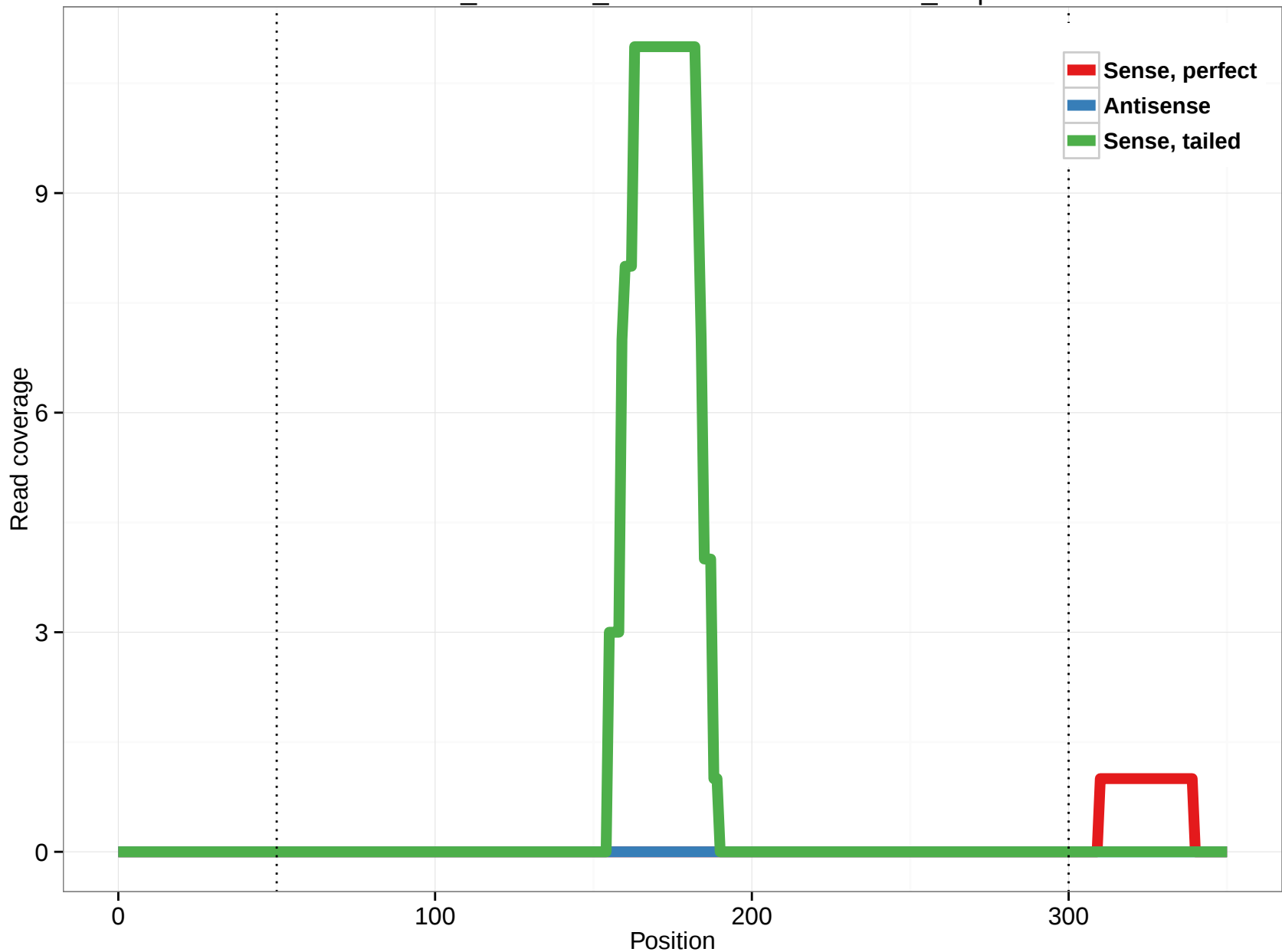
ornAna1_ensGene_ENSOANT00000014687_7.3p
