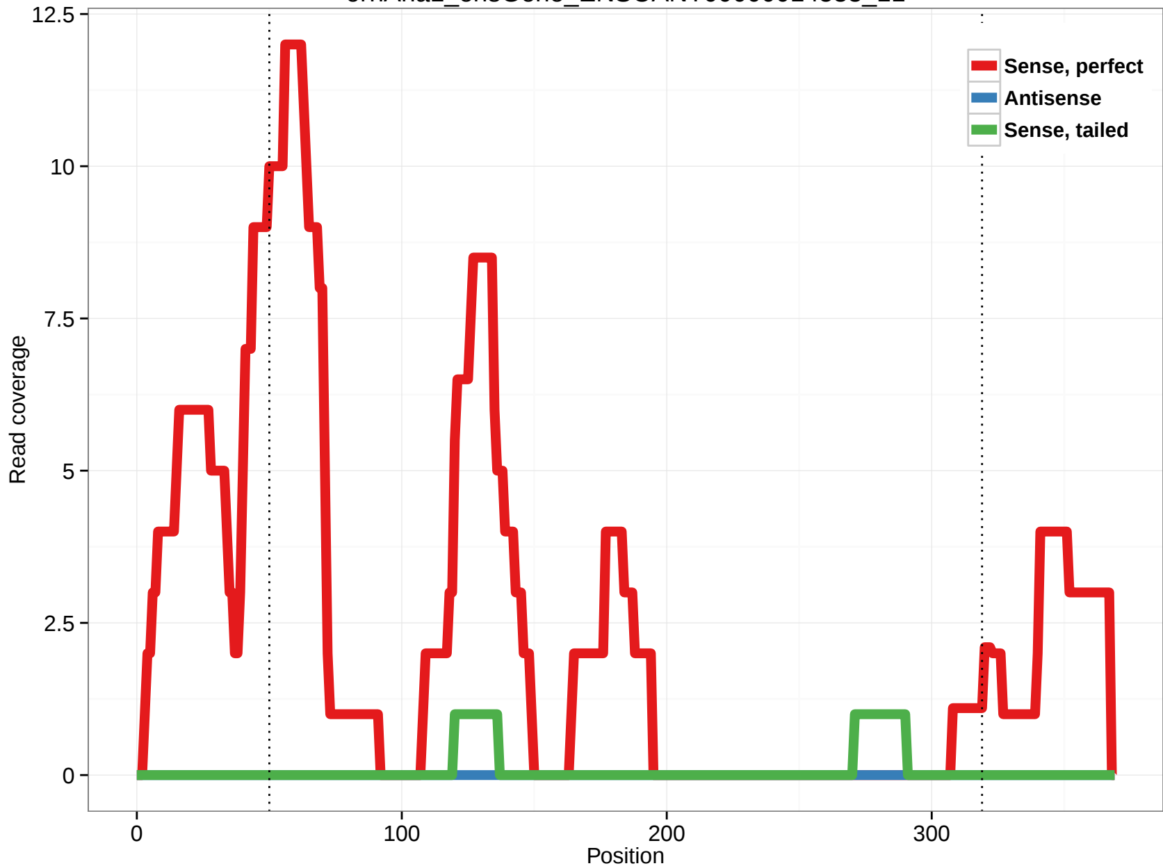
ornAna1_ensGene_ENSOANT00000014533_11
