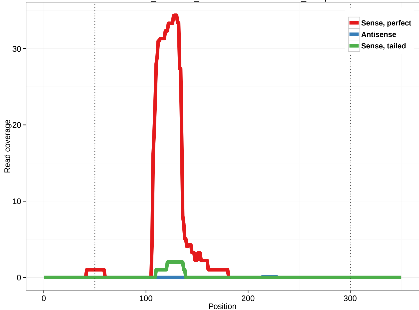
ornAna1_ensGene_ENSOANT00000014474_13.3p
