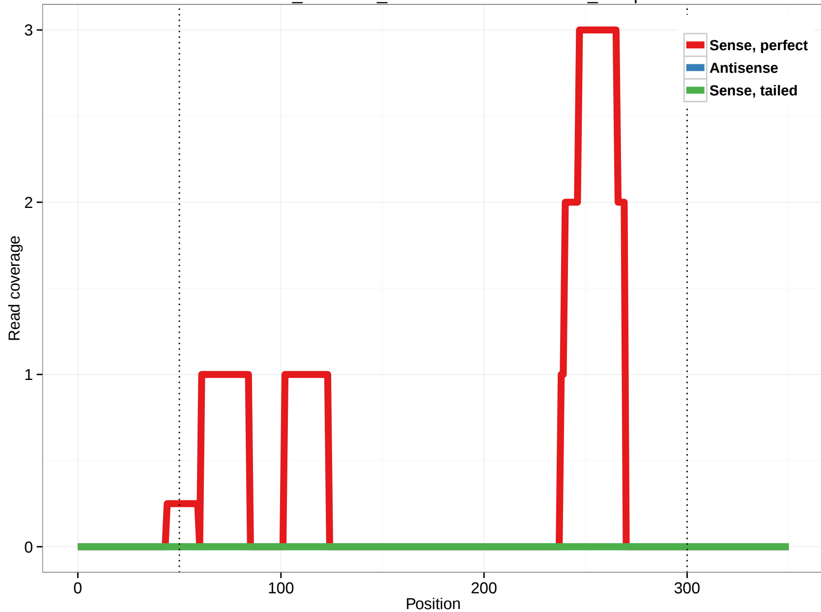
ornAna1_ensGene_ENSOANT00000014444_10.3p
