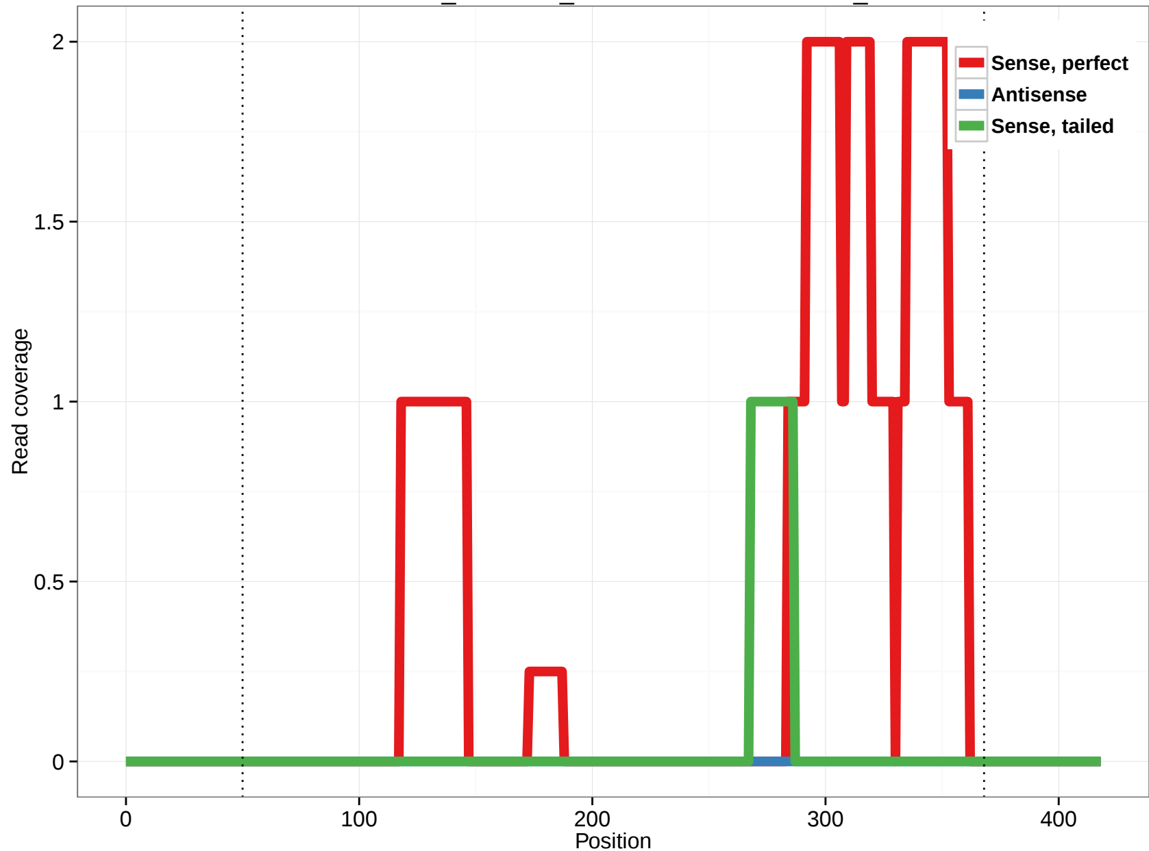
ornAna1_ensGene_ENSOANT00000014439_1
