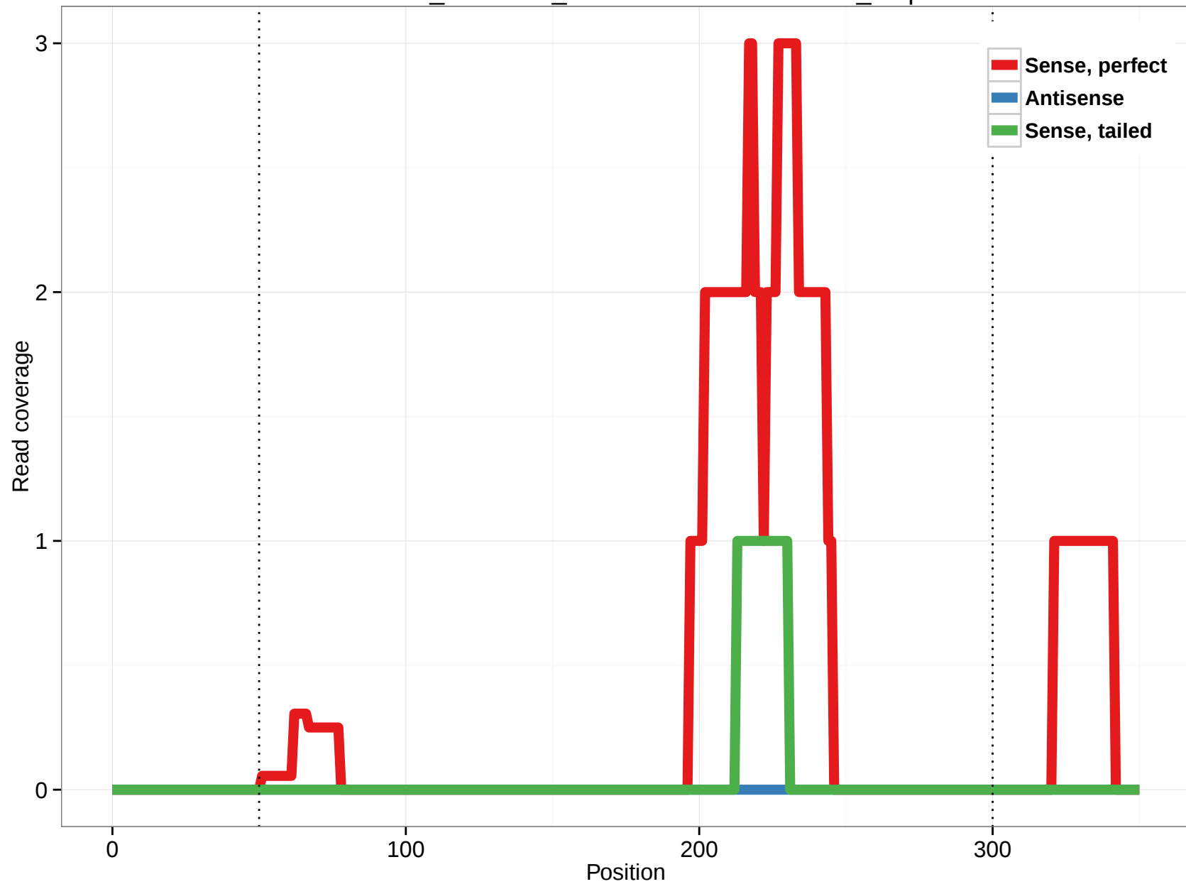
ornAna1_ensGene_ENSOANT00000014368_2.3p
