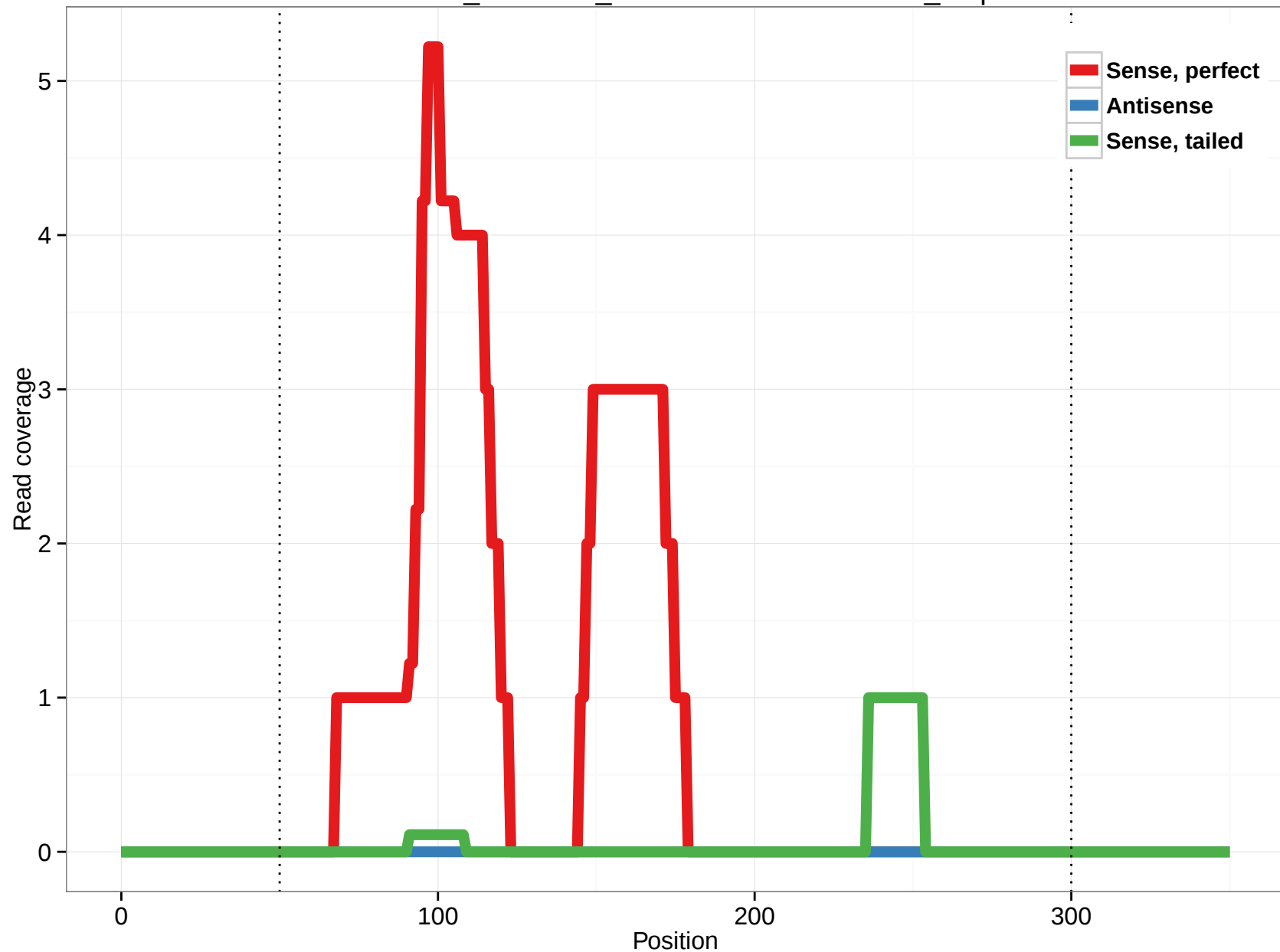
ornAna1_ensGene_ENSOANT00000014350_5.5p
