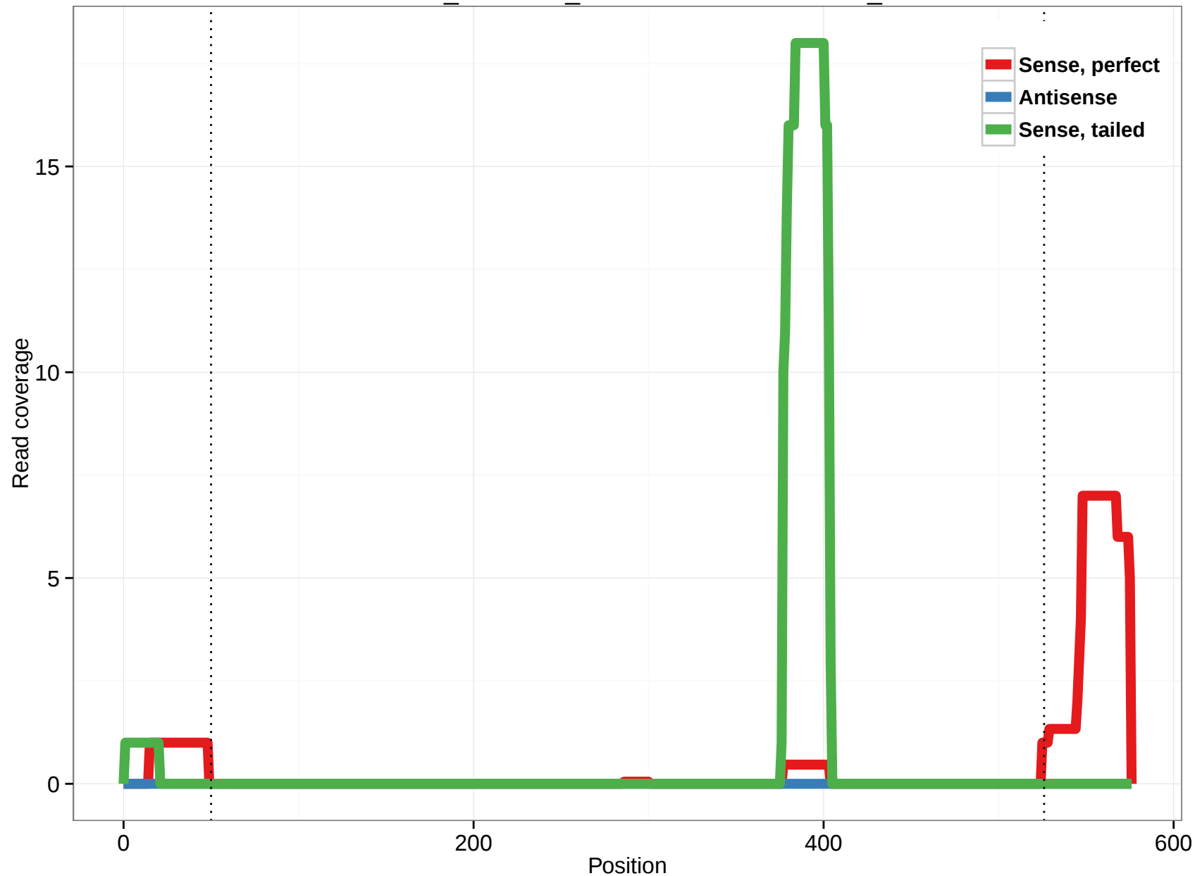
ornAna1_ensGene_ENSOANT00000014287_12
