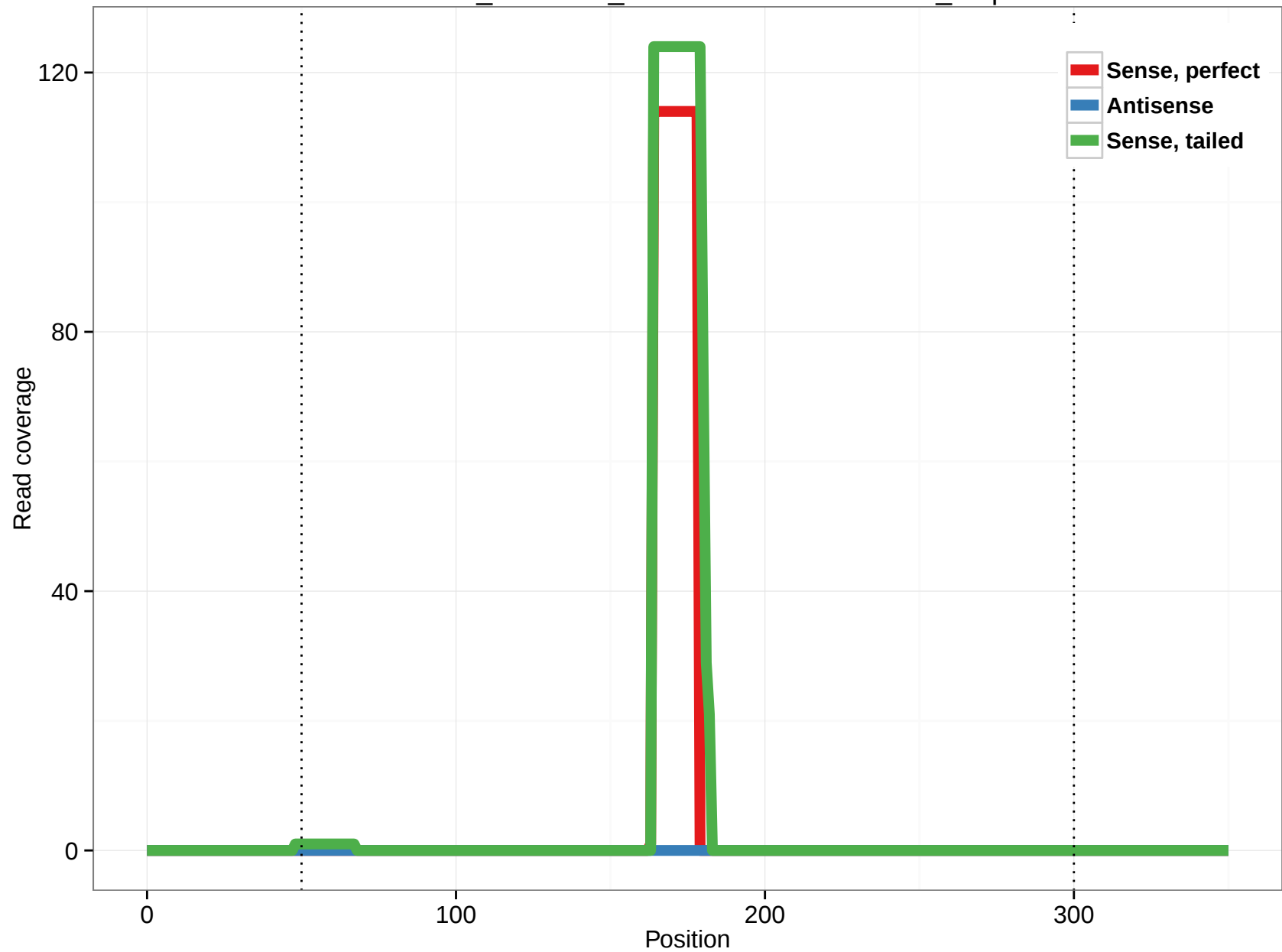
ornAna1_ensGene_ENSOANT00000014192_8.5p
