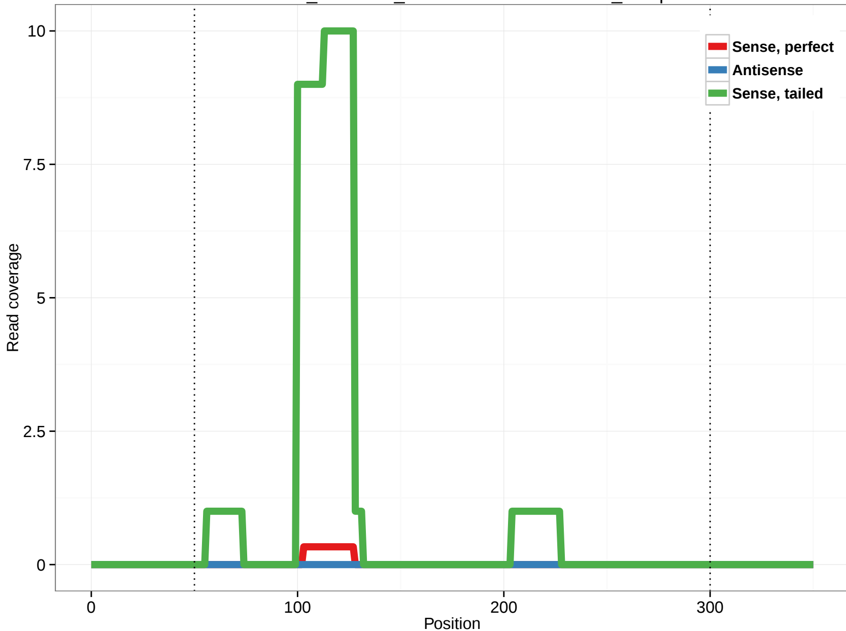
ornAna1_ensGene_ENSOANT00000014115_14.3p
