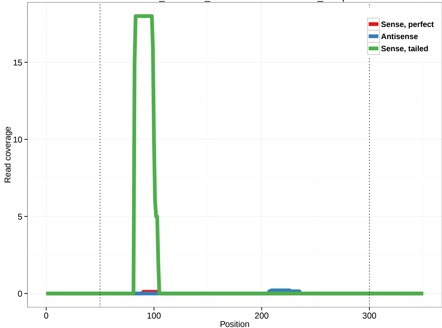
ornAna1_ensGene_ENSOANT00000014089_25.3p
