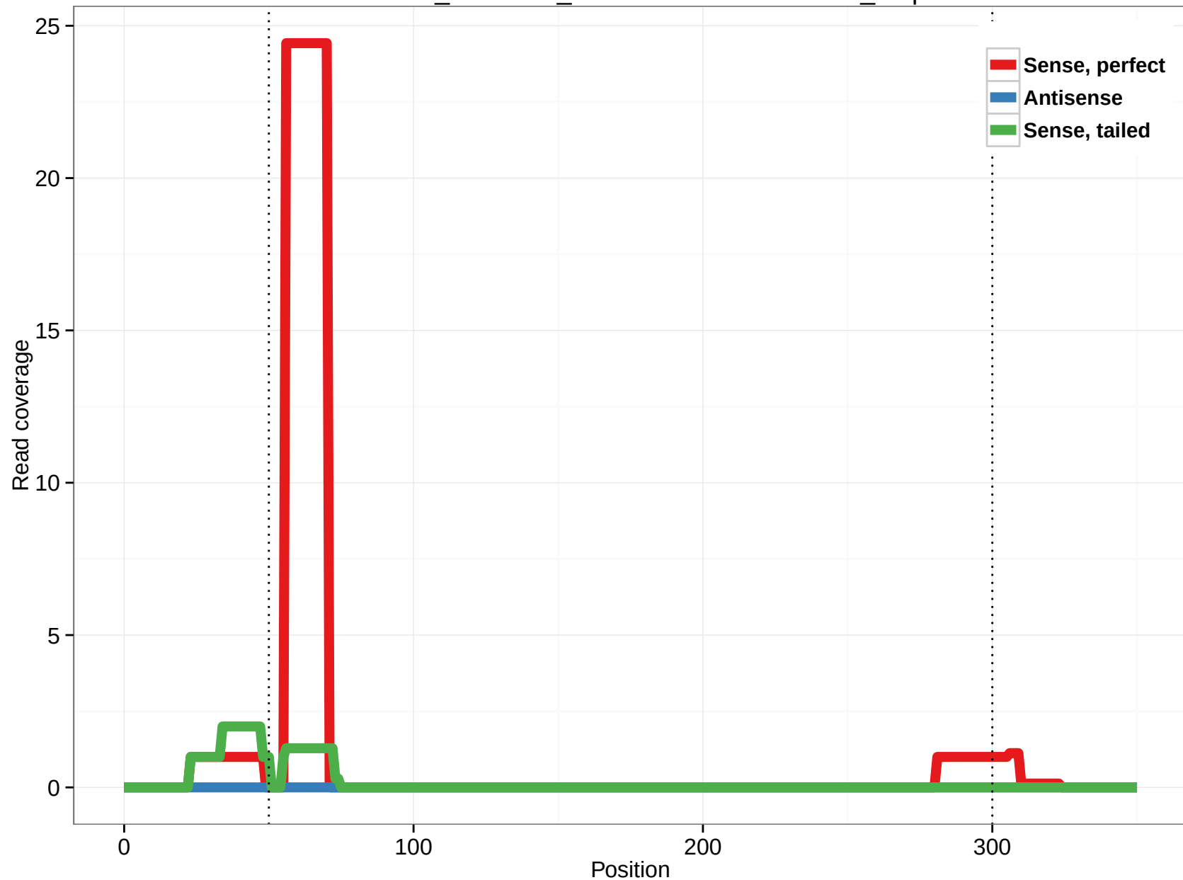
ornAna1_ensGene_ENSOANT00000014036_8.5p
