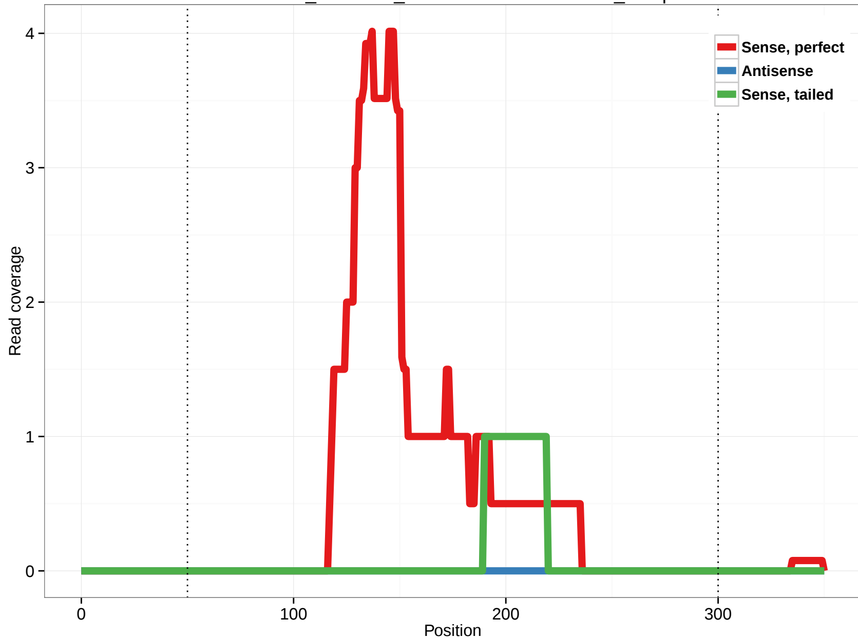
ornAna1_ensGene_ENSOANT00000014017_13.3p
