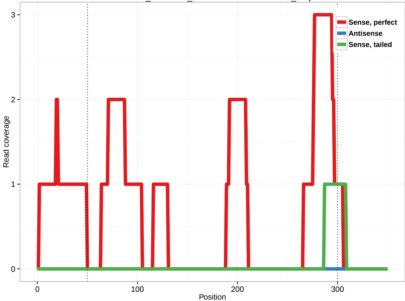
ornAna1_ensGene_ENSOANT00000014008_6.5p
