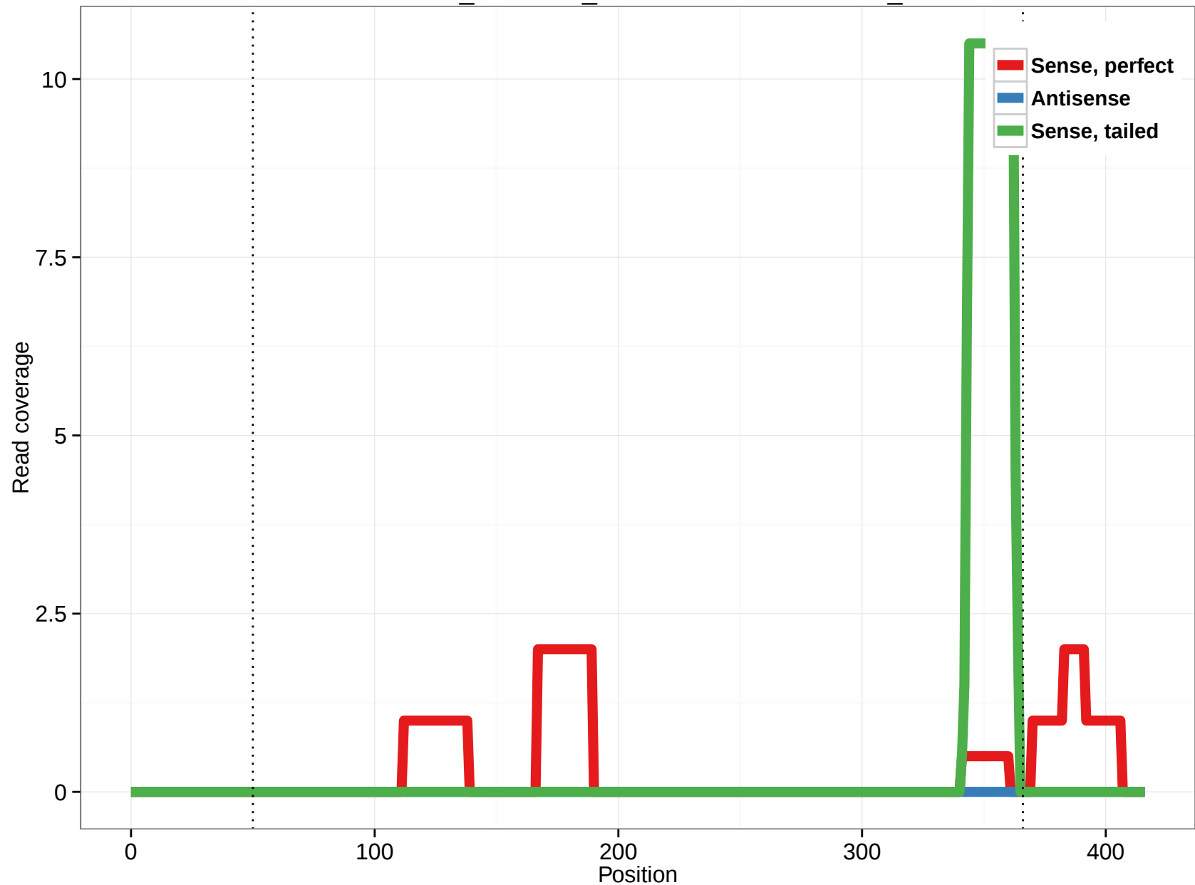
ornAna1_ensGene_ENSOANT00000013999_4
