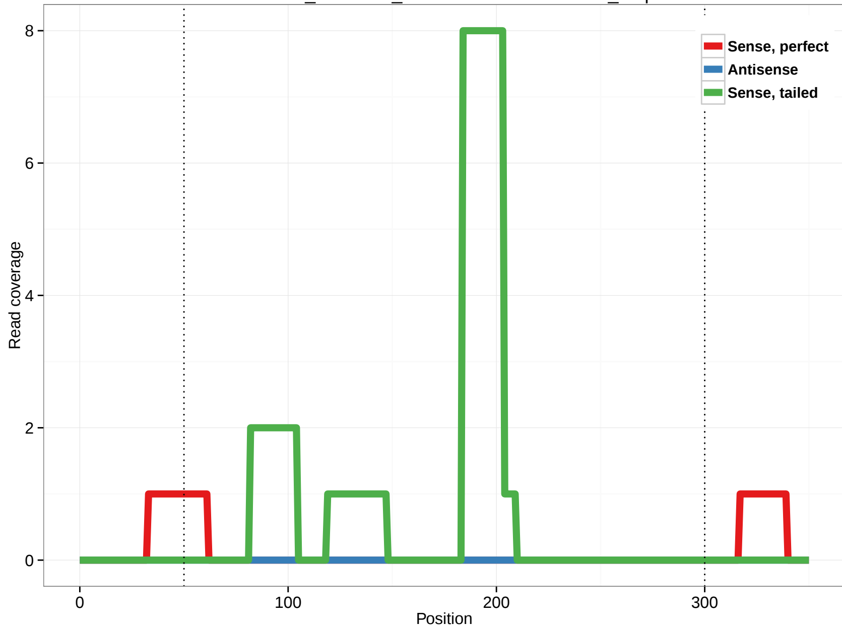
ornAna1_ensGene_ENSOANT00000013968_9.3p
