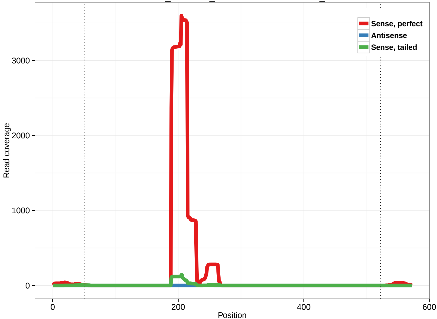
ornAna1_ensGene_ENSOANT00000013919_10
