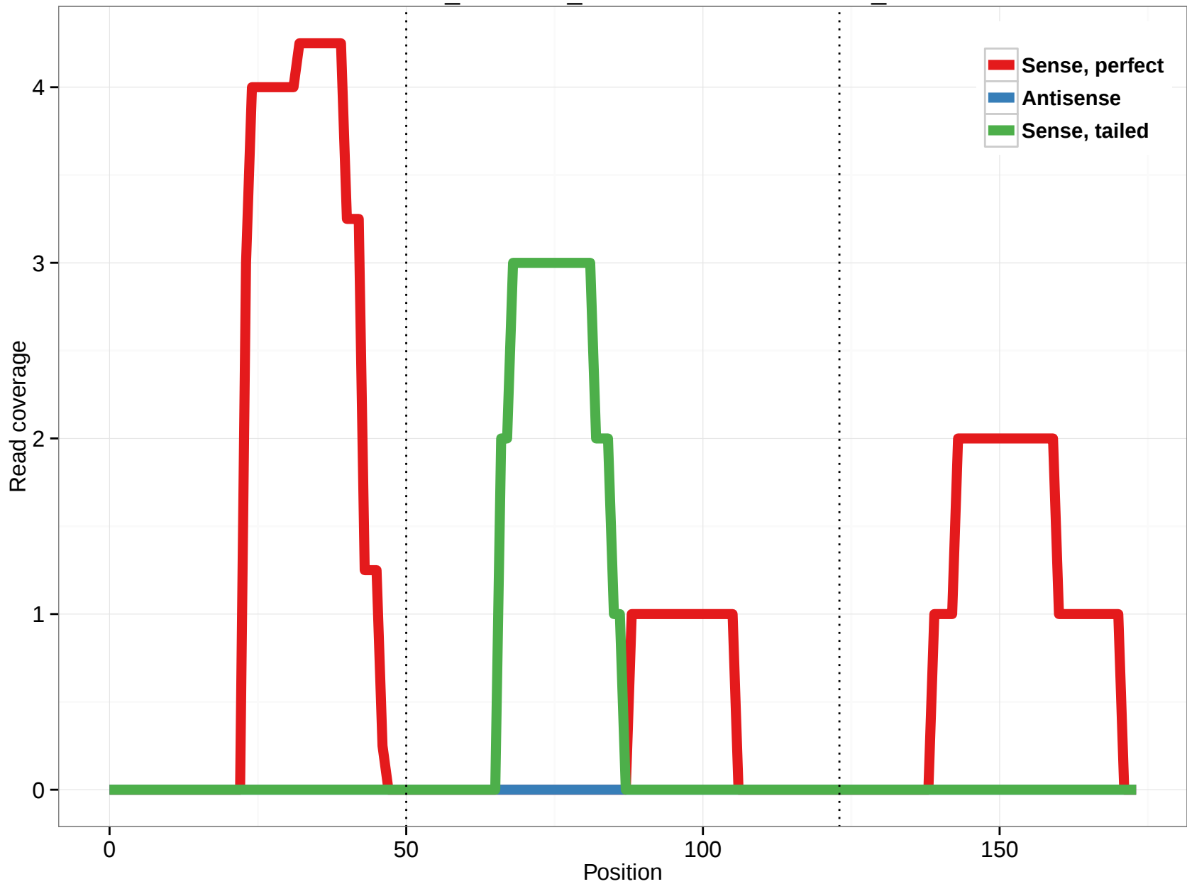
ornAna1_ensGene_ENSOANT00000013800_2
