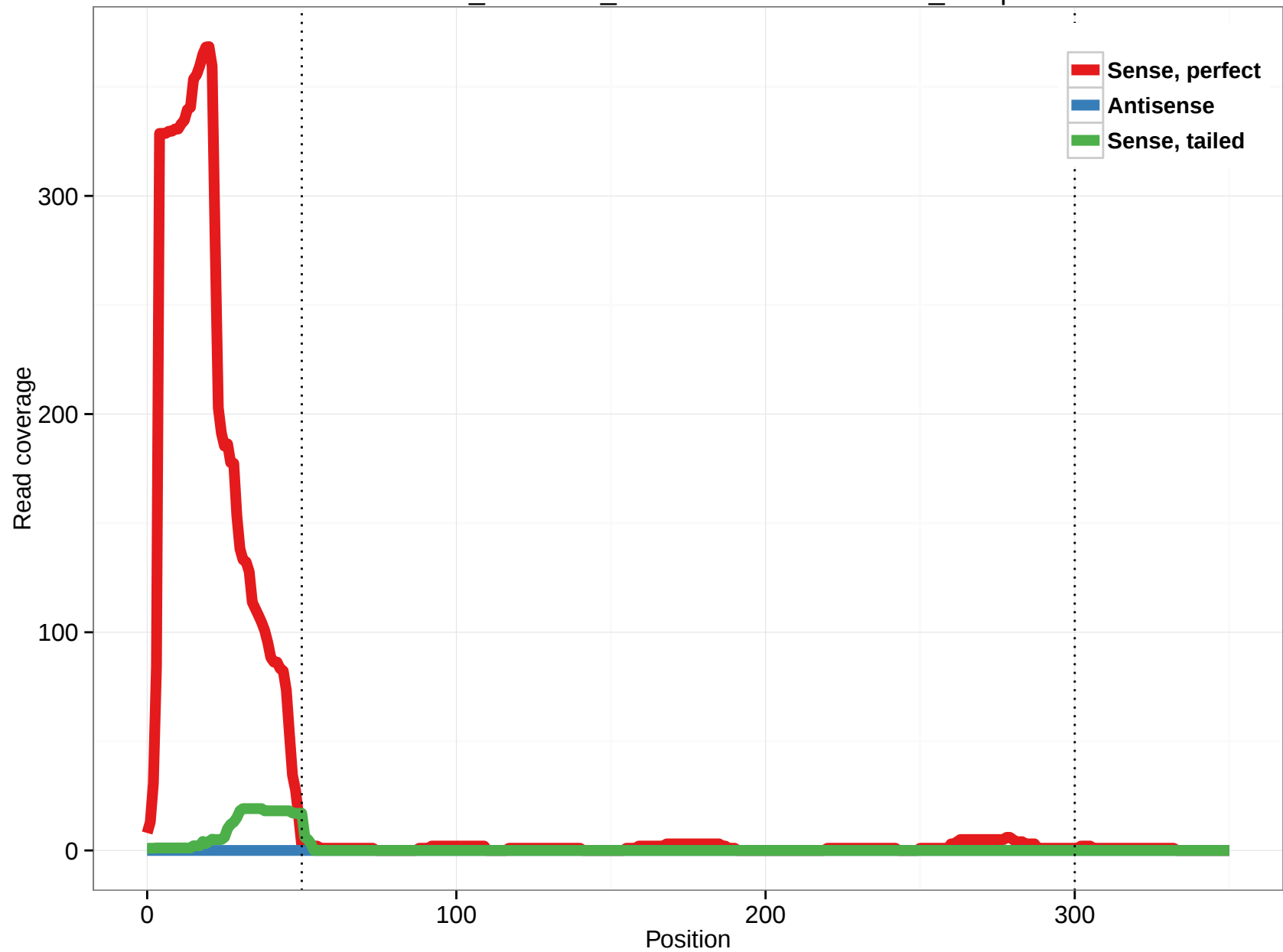
ornAna1_ensGene_ENSOANT00000013779_44.5p
