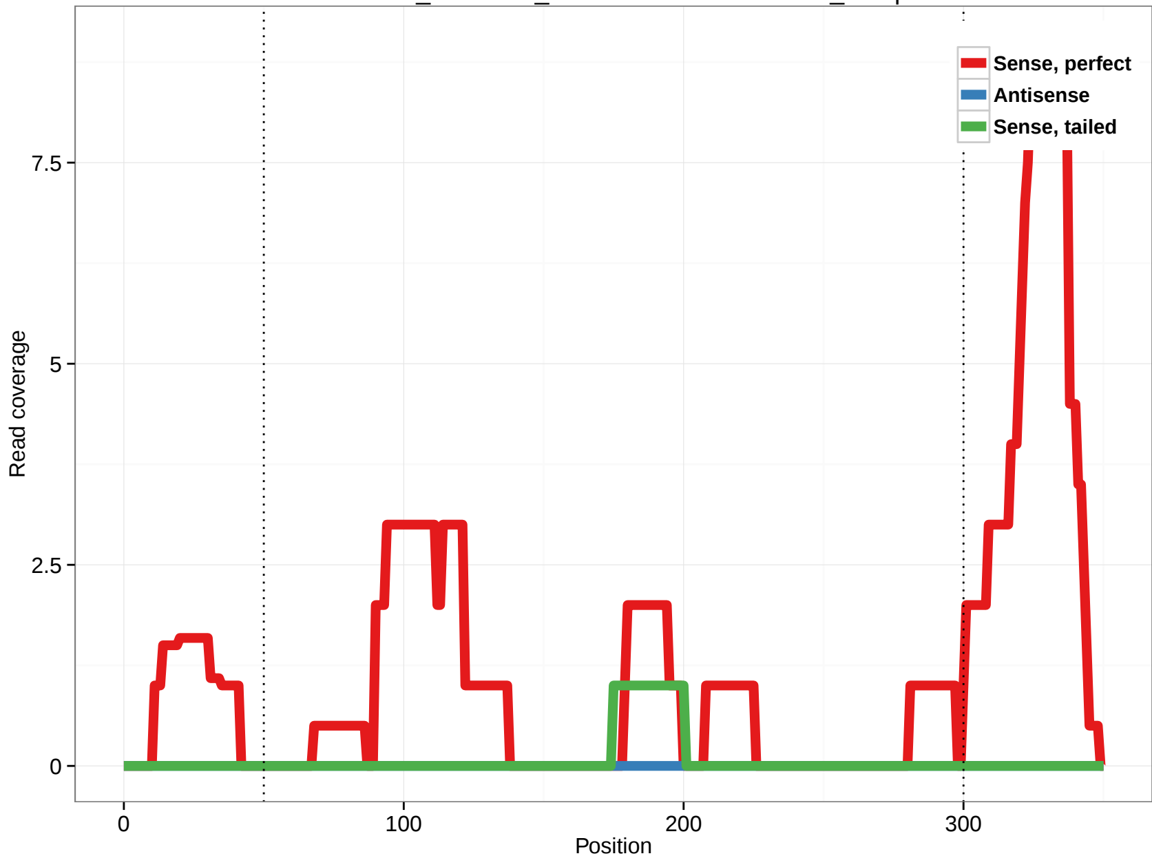
ornAna1_ensGene_ENSOANT00000013779_44.3p
