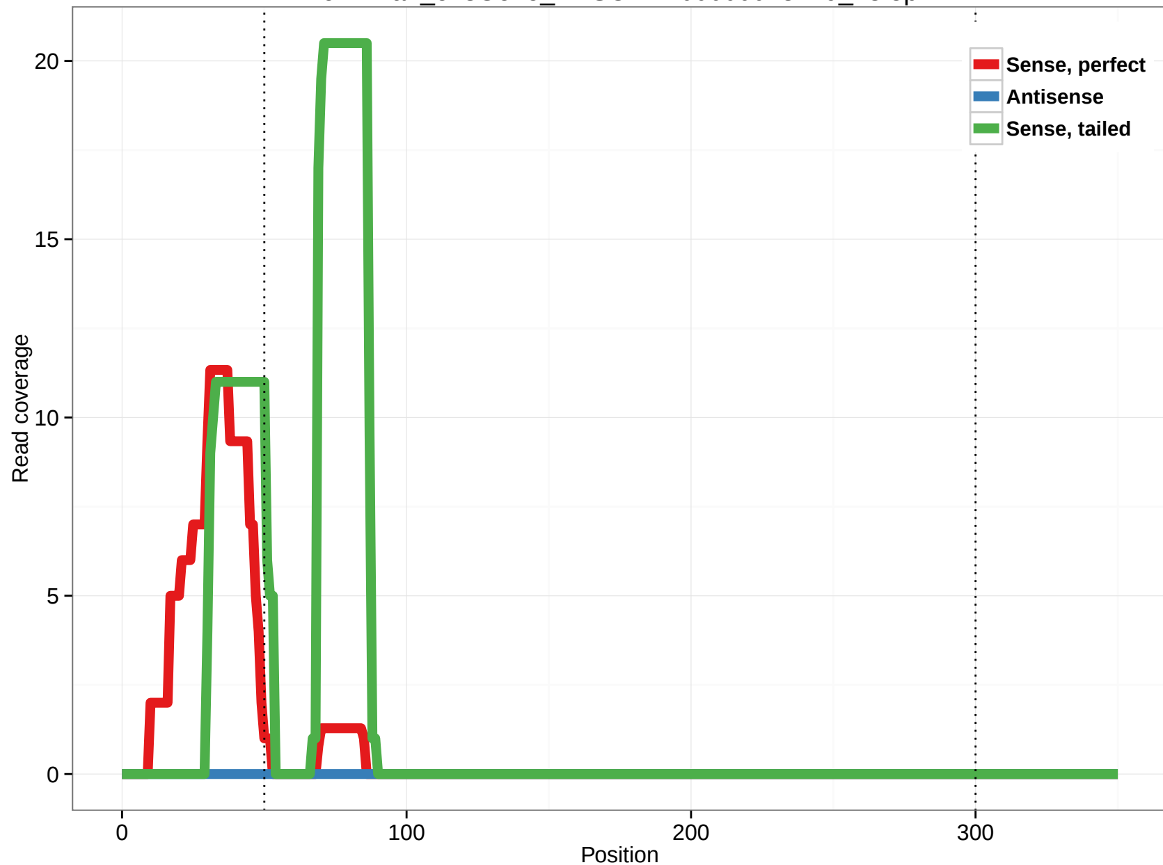
ornAna1_ensGene_ENSOANT00000013779_43.5p
