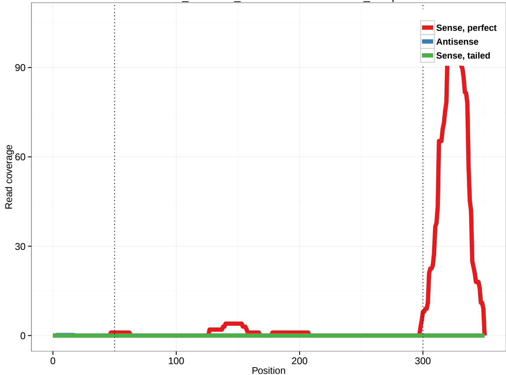
ornAna1_ensGene_ENSOANT00000013777_60.3p
