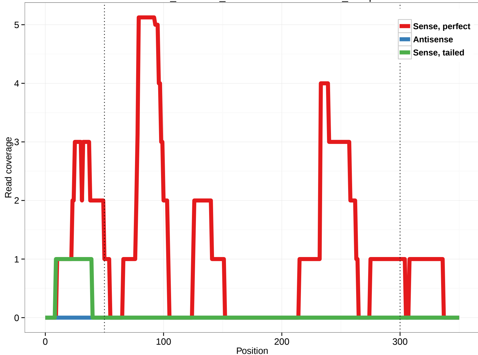
ornAna1_ensGene_ENSOANT00000013777_51.5p
