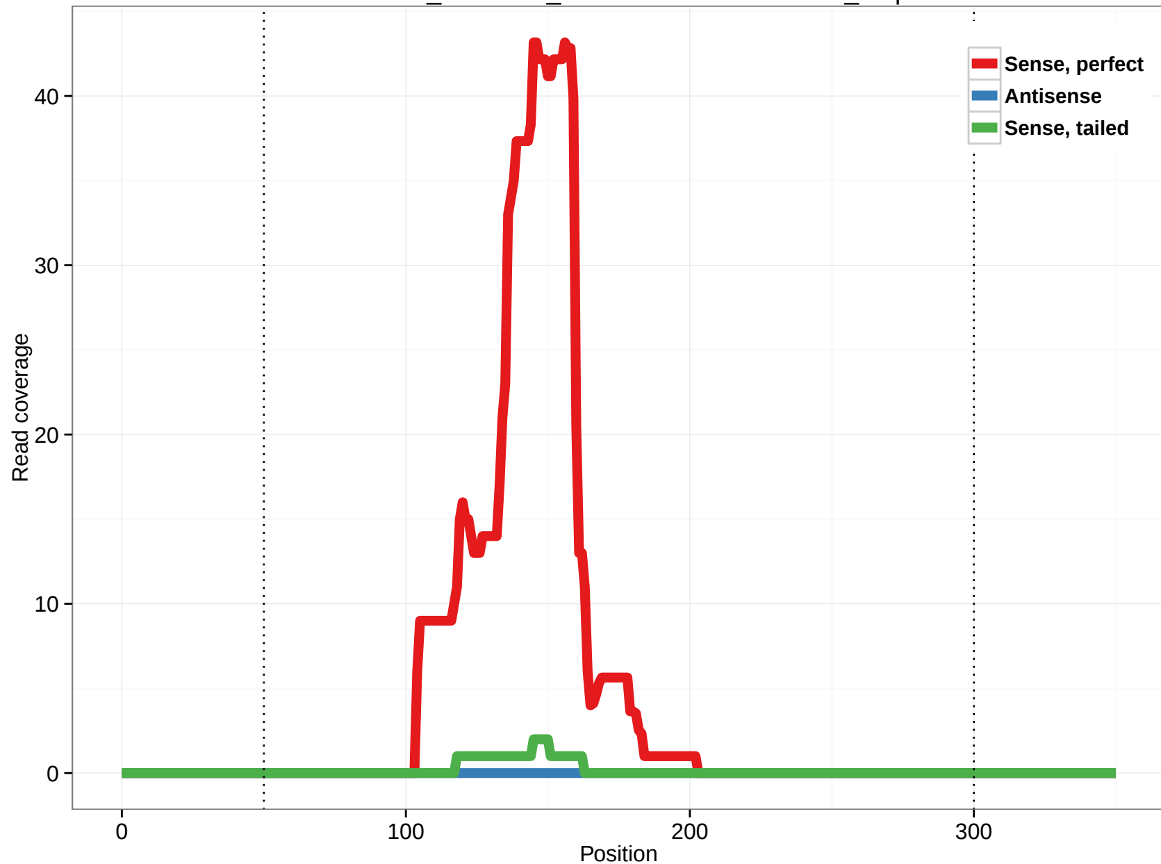
ornAna1_ensGene_ENSOANT00000013768_9.5p
