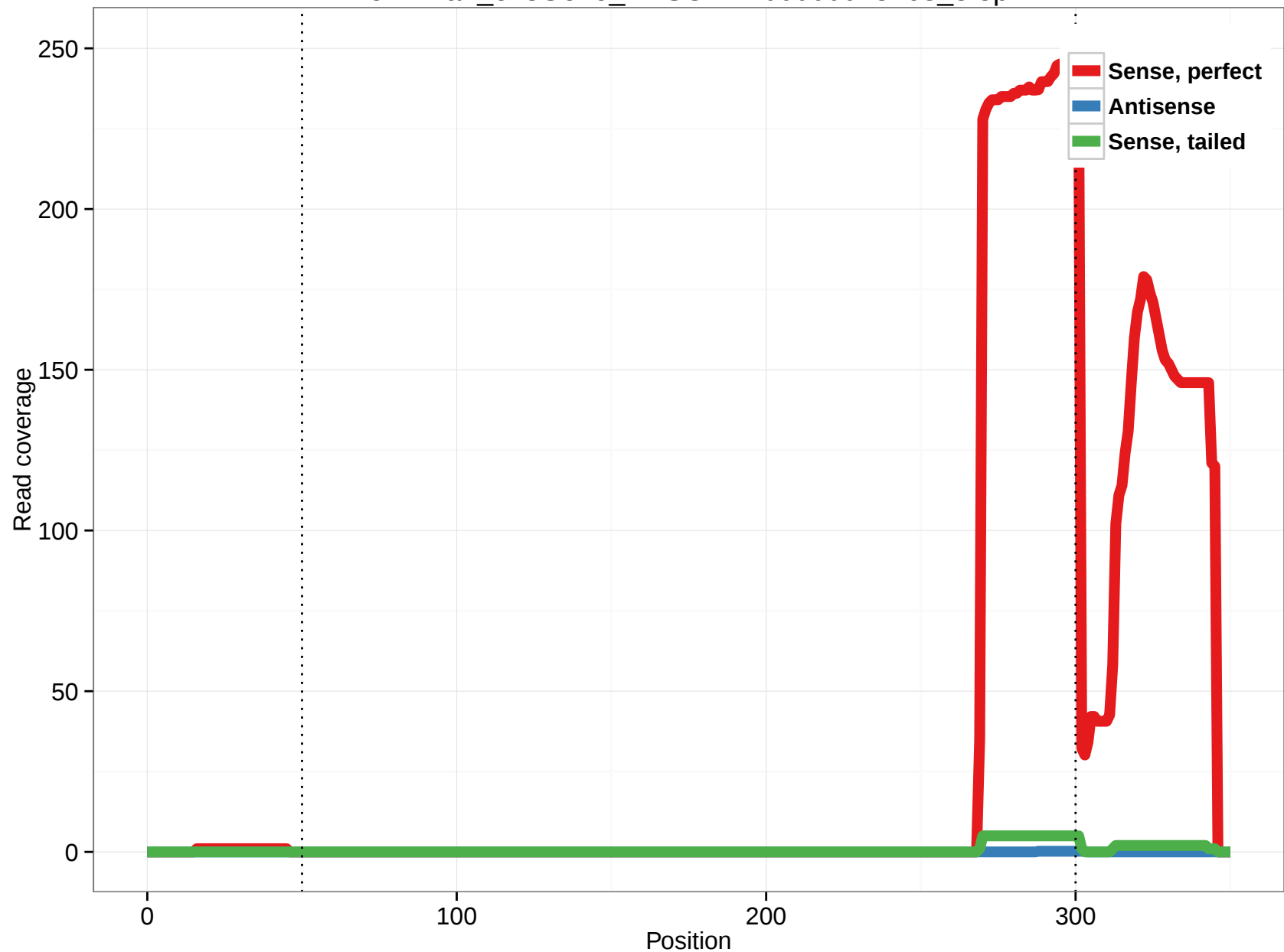
ornAna1_ensGene_ENSOANT00000013768_8.5p
