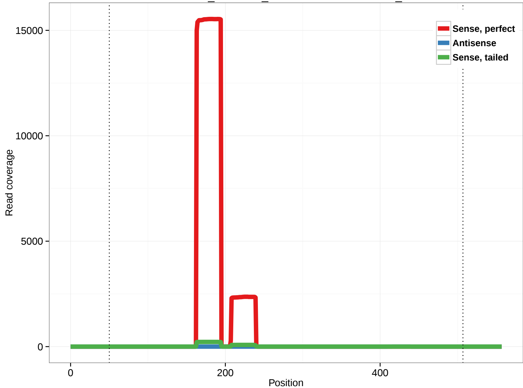
ornAna1_ensGene_ENSOANT00000013768_7
