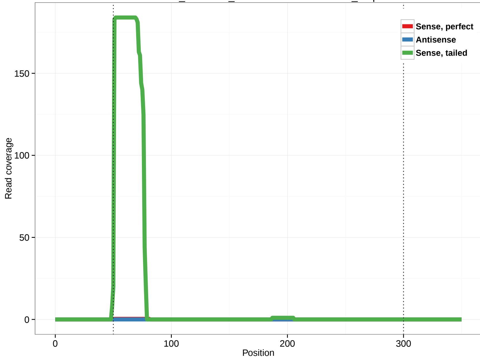
ornAna1_ensGene_ENSOANT00000013692_0.5p
