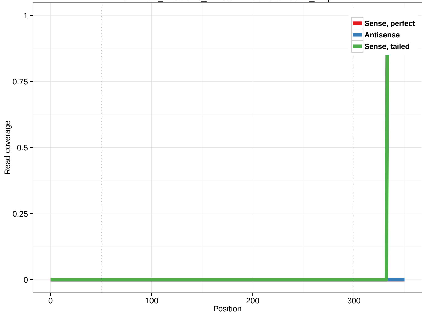
ornAna1_ensGene_ENSOANT00000013627_0.3p
