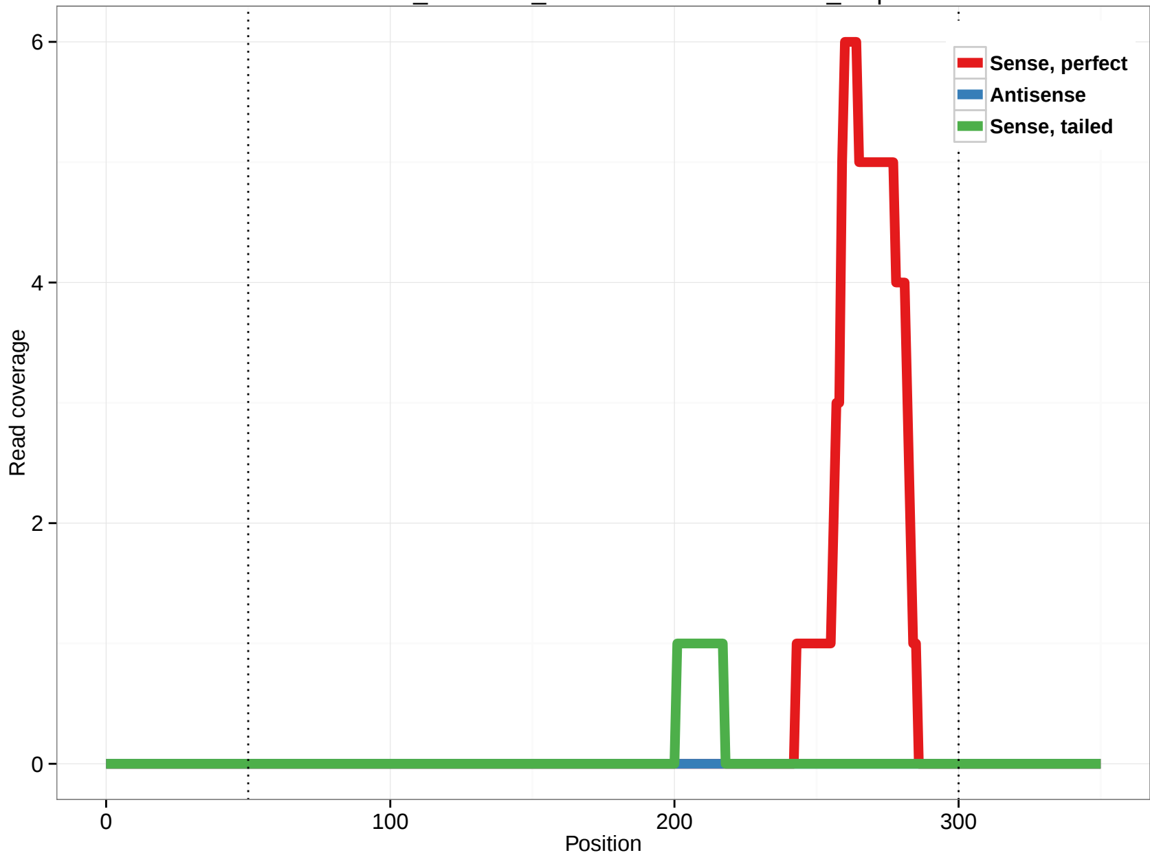
ornAna1_ensGene_ENSOANT00000013609_4.5p
