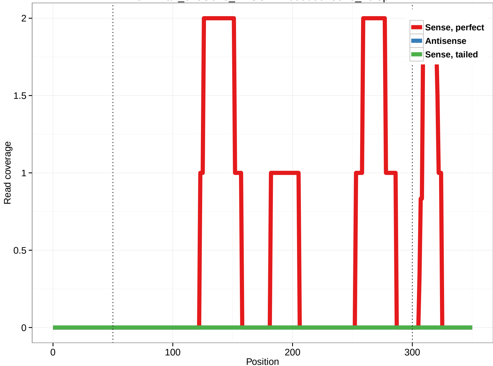
ornAna1_ensGene_ENSOANT00000013576_20.3p
